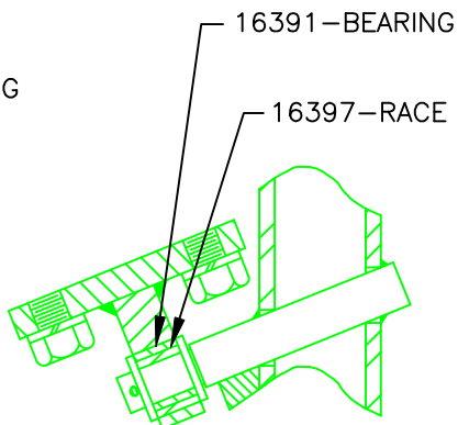
DETAIL "E"
