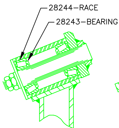
DETAIL "D"
